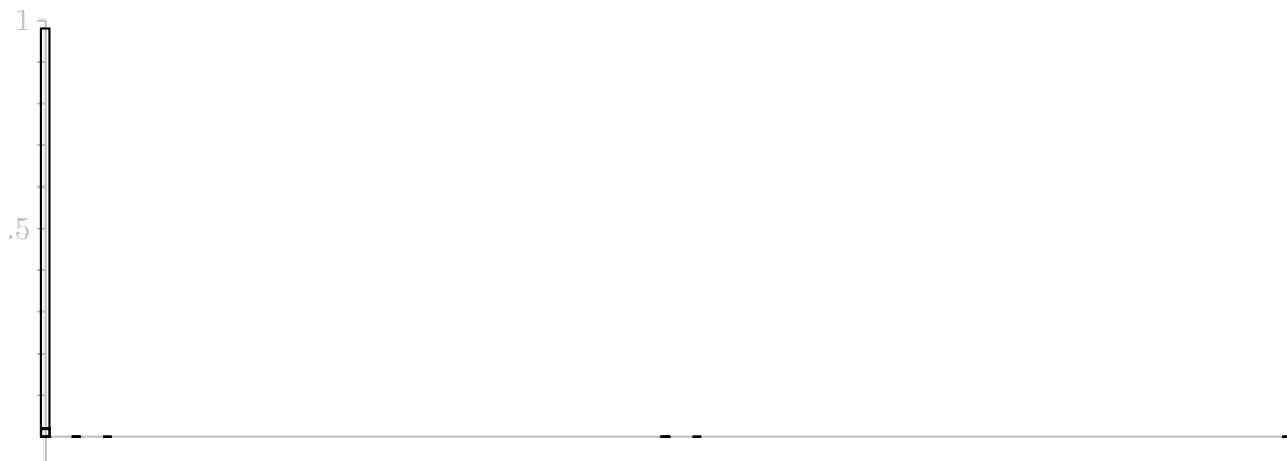
Average of two draws
