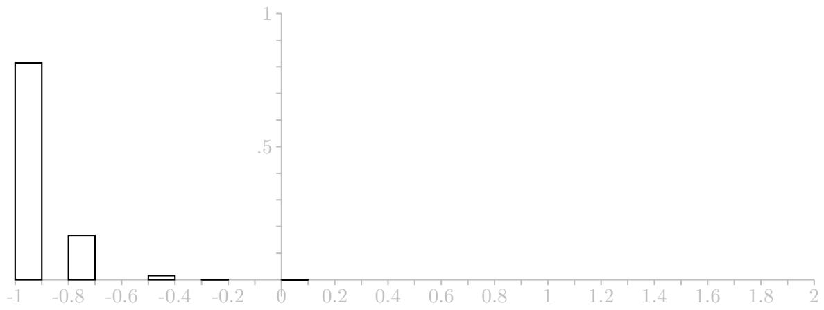
Average of 20 draws
