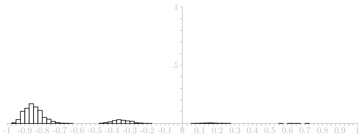
Average of 20000 draws
