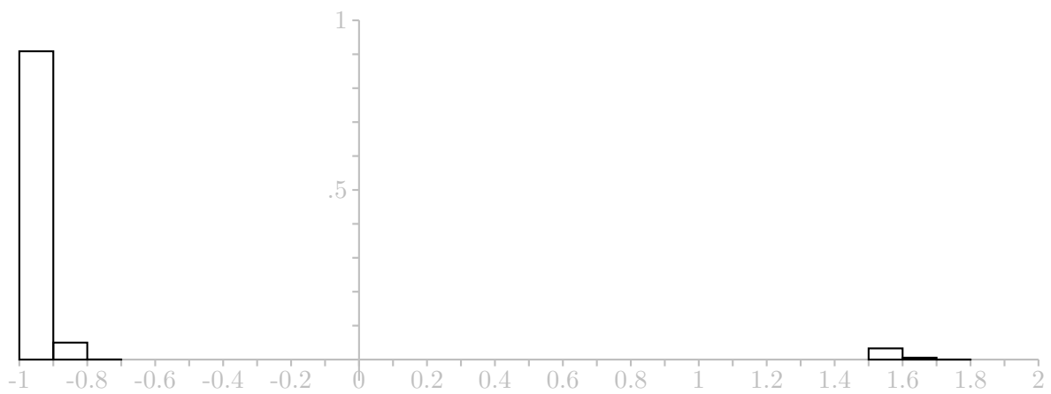
Average of 200 draws
