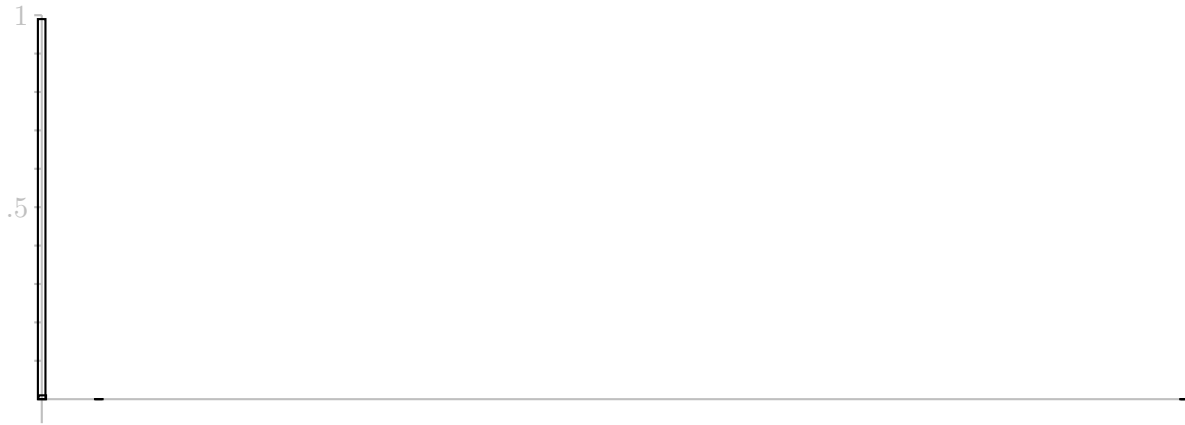
Average of one draw
