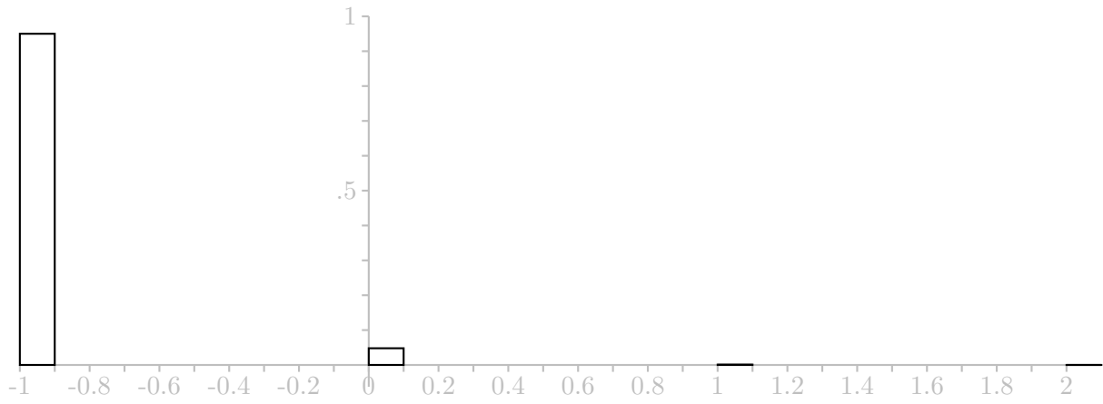
Average of 5 draws
