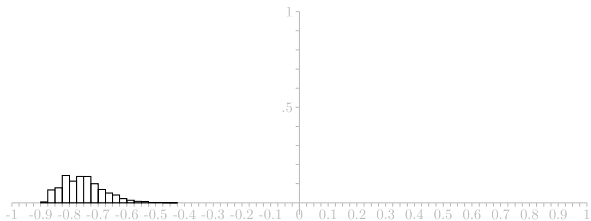
Average of 200000 draws
