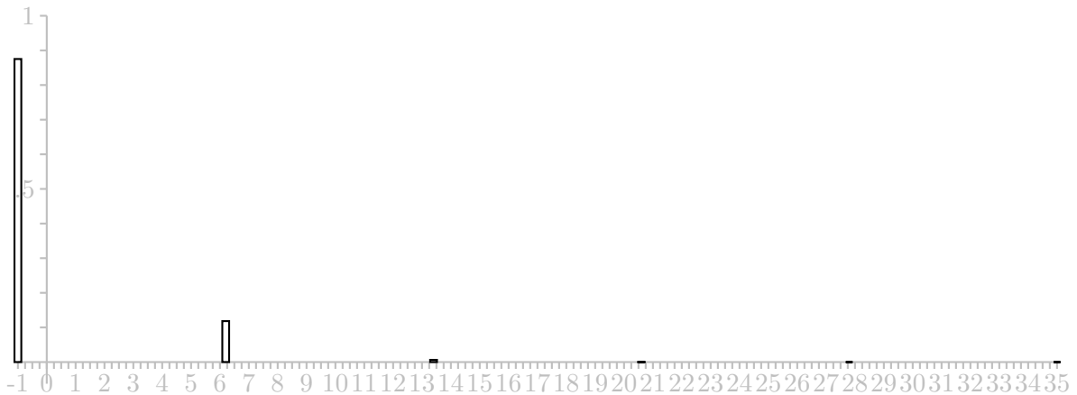
Bob's Strategy — Average of 5 draws
