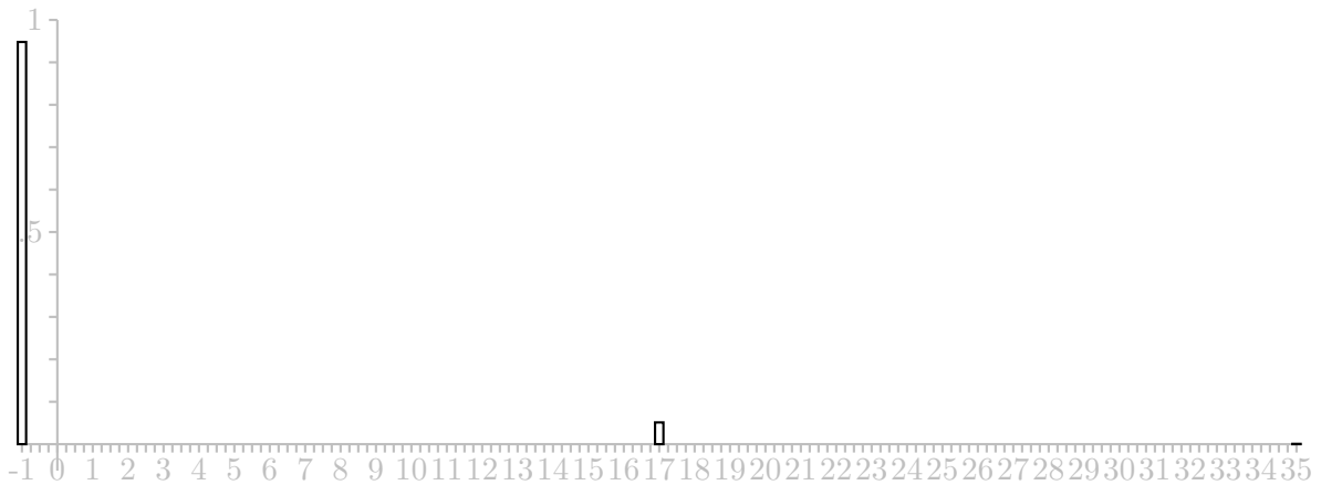
Bob's Strategy — Average of two draws
