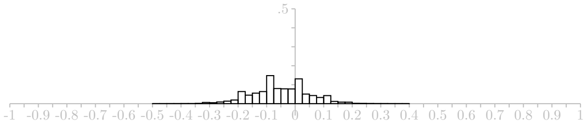
Alice's Strategy — Average of 100 draws
