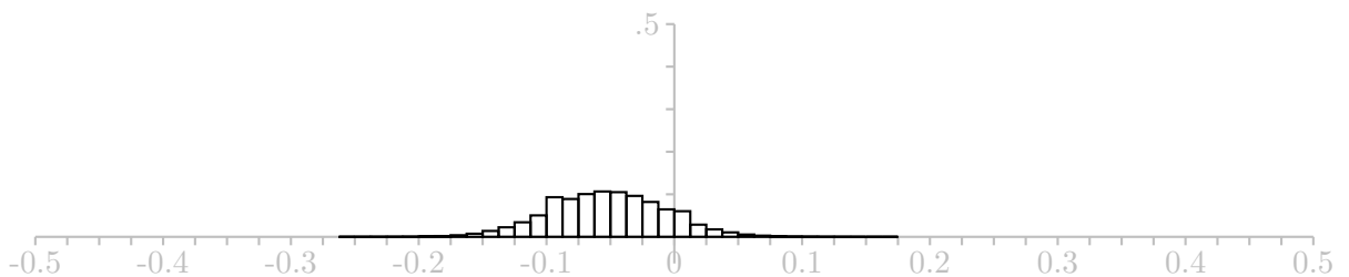
Alice's Strategy — Average of 500 draws
