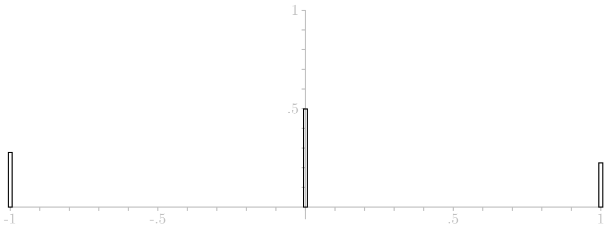
Alice's Strategy — Average of two draws
