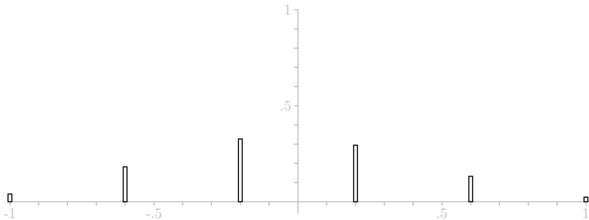
Alice's Strategy — Average of 5 draws
