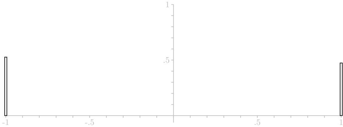
Alice's Strategy — One Draw
