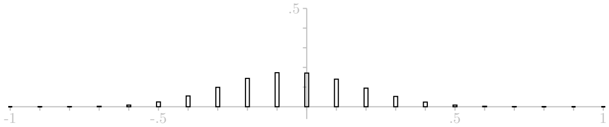
Alice's Strategy — Average of 20 draws
