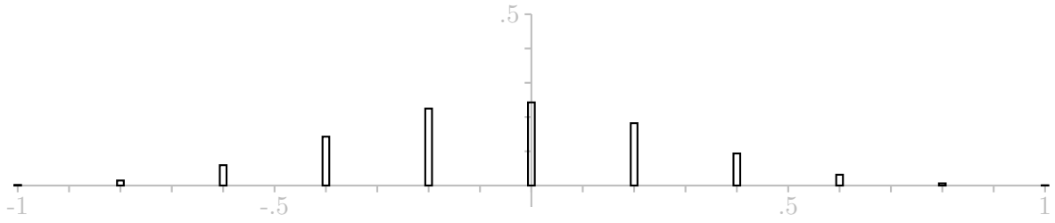
Alice's Strategy — Average of 10 draws
