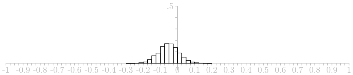
Bob's Strategy — Average of 10000 draws
